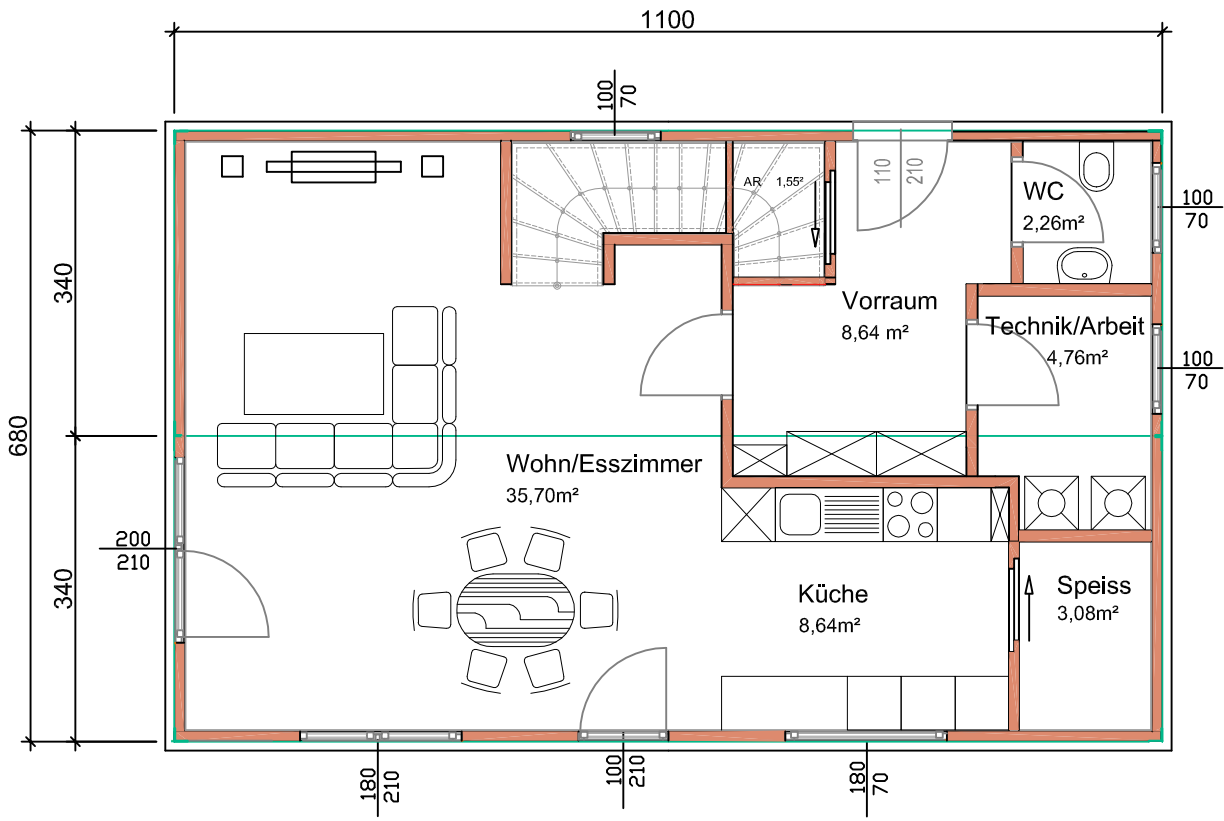
Erdgeschoss WNFL 64,63 m 2
